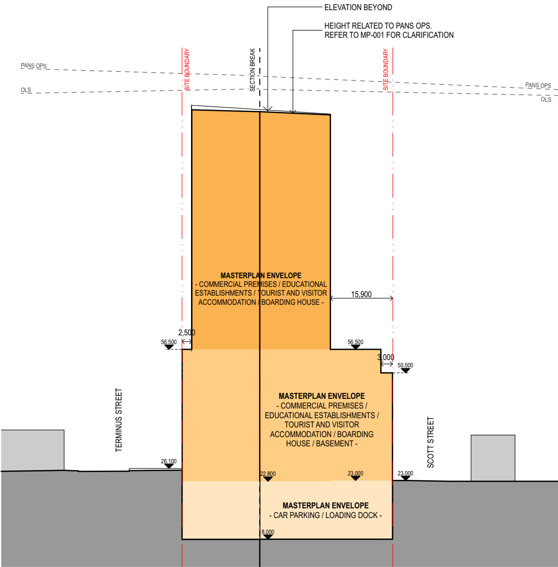
SECTION C
