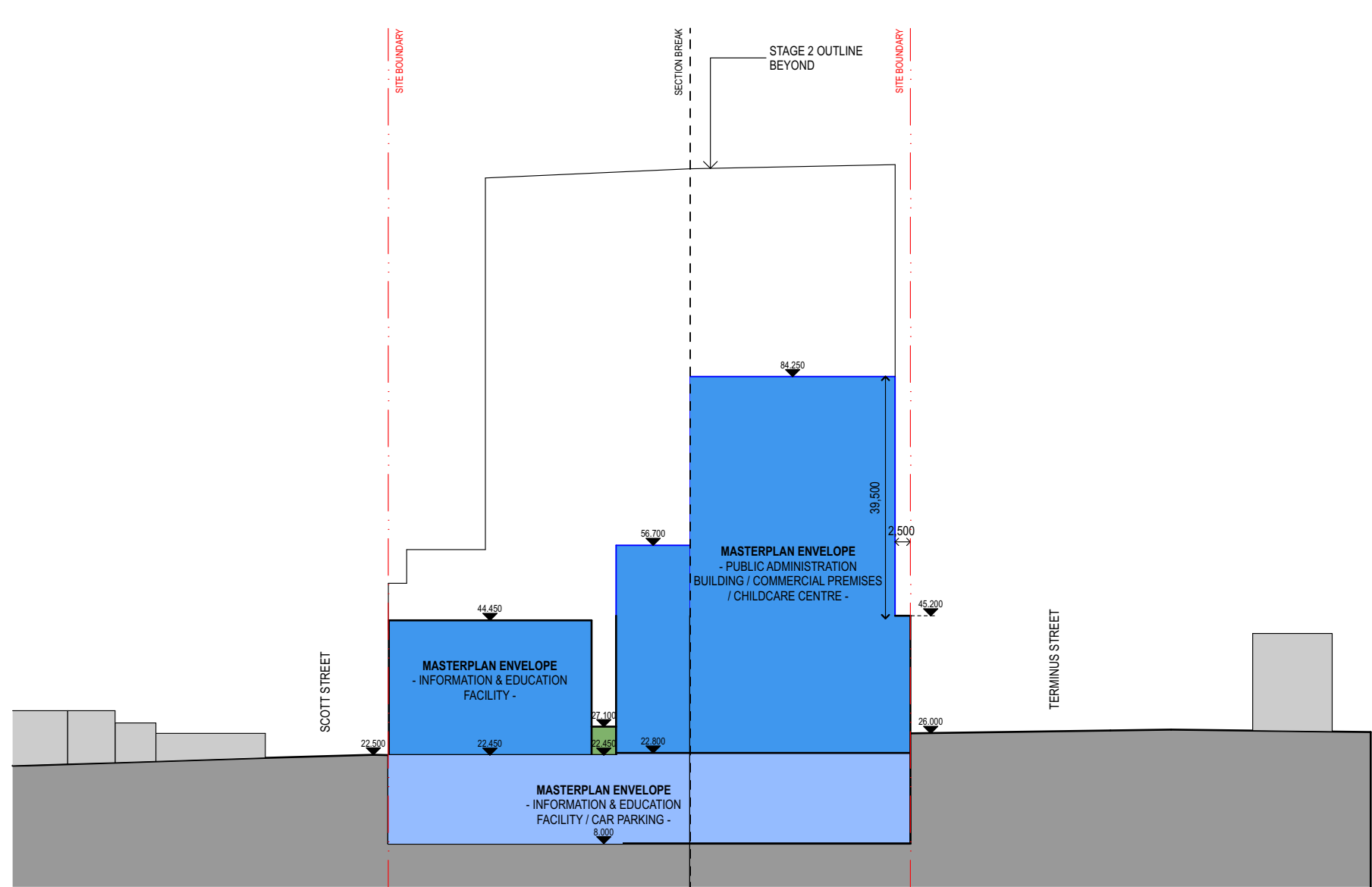
SECTION B
